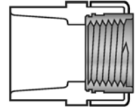
Transition Female Adapter Soc x Fipt With Brass Thread Insert
